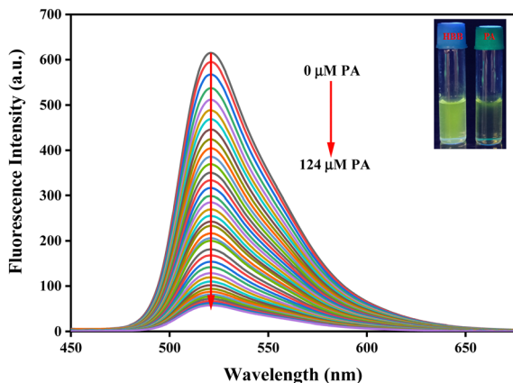
Fig. 9 Fluorescence titration spectra ( \lambda_{\text{ex}} = 365 \text{ nm} ) of fluorescent MBB microparticles (comprising 99% water) while introducing various concentrations of PA. Inset: Visualization of the change from robust green color fluorescence to non-fluorescence in the presence of PA.
