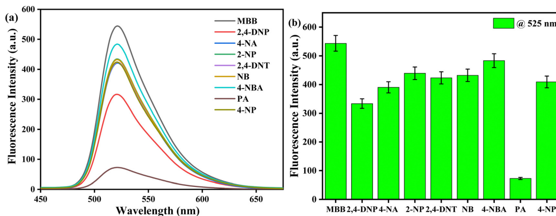
Fig. 10 (a) Emission spectra ( \lambda_{\text{ex}} = 365 \text{ nm} ) of MBB microparticles with several NACs. (b) Bar plot of fluorescence quenching of MBB microparticles after the addition of various NACs.
