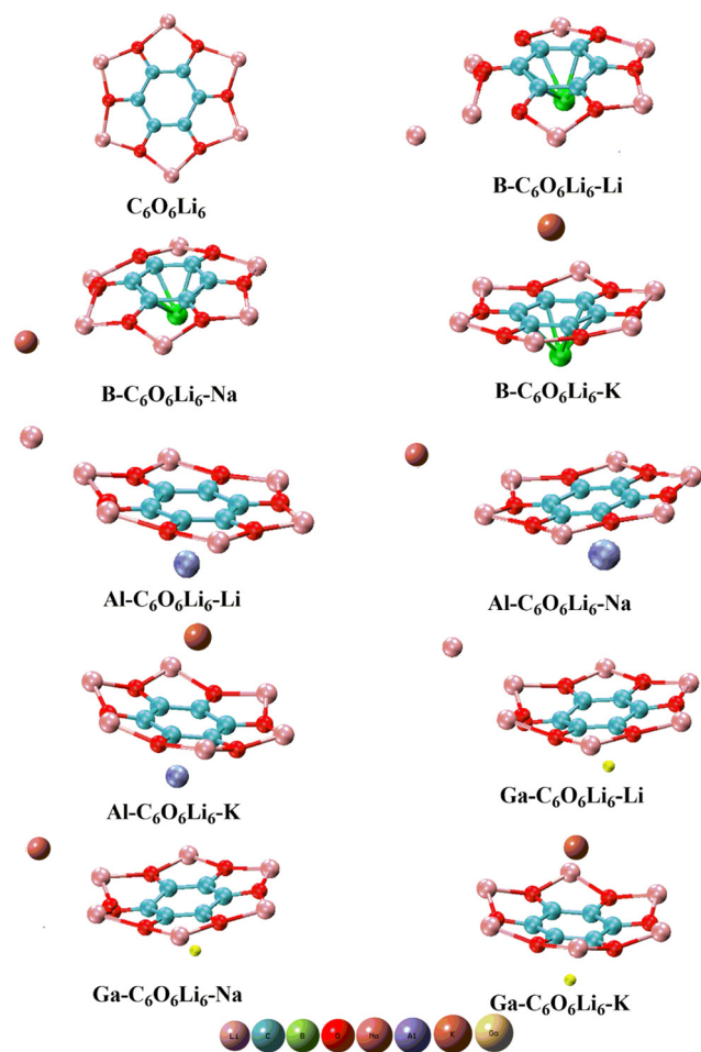
Fig. 1 Pristine \text{C}_6\text{O}_6\text{Li}_6 and group-IA and group-IIIA metal-doped \text{C}_6\text{O}_6\text{Li}_6 complexes.
