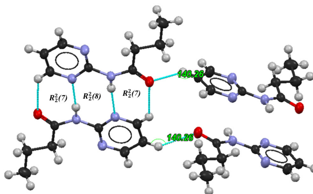
Fig. 5 The intermolecular interactions in three different types of single crystal structures appeared in the PM series.
