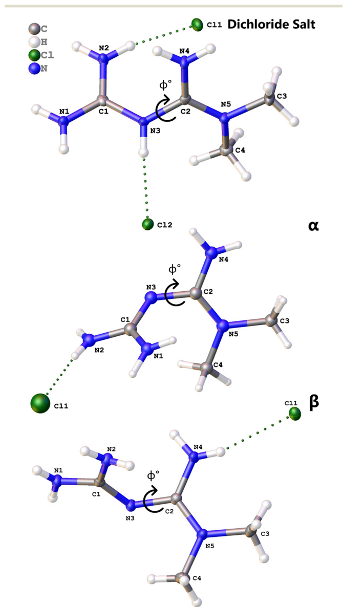
Fig. 1 Asymmetric unit of (top) metformin dihydrochloride, (middle) \alpha -metformin hydrochloride and (bottom) \beta -metformin hydrochloride. 21,22
