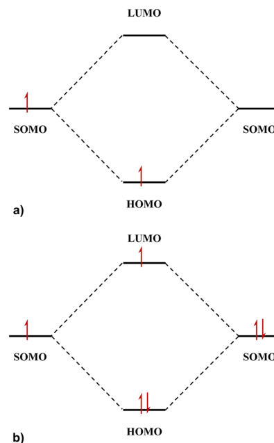
Fig. 4 A schematic representation of orbitals in a bond with an order of 1/2: a) a single bonding electron in a dimer of PLY-PLY + , 48 and b) two bonding electrons and one antibonding electron in a close contact of TCNQ-TCNQ - . 51
