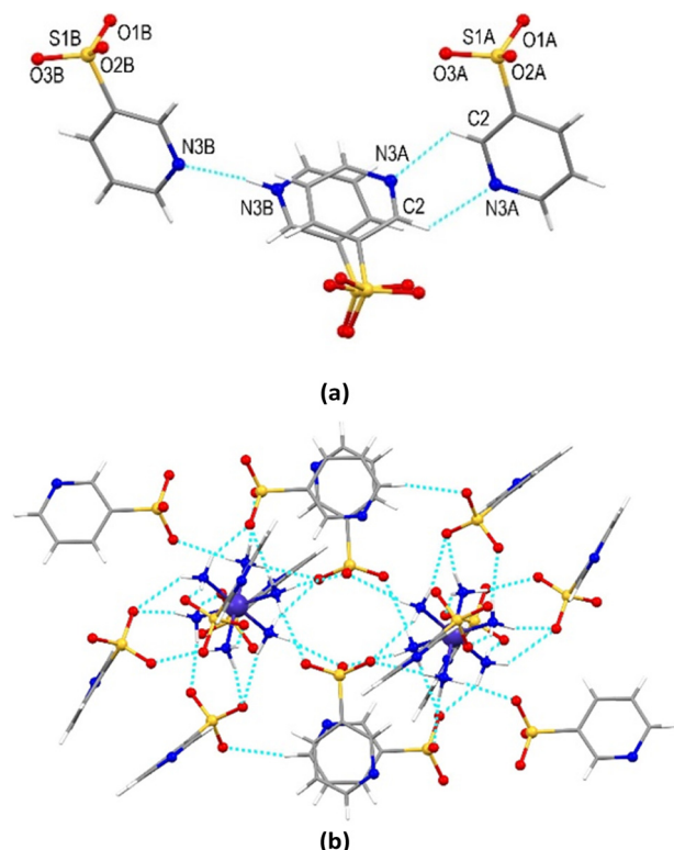
Fig. 1 (a) The H-bonds between the disordered \text{pys}^- anions and the neutral Hpys molecule in 1 . (b) H-bonding interactions around [\text{Co}(\text{NH}_3)_6]^{3+} cations in the structure of 1 . Hydrogen bonds are shown as blue dashed lines.
