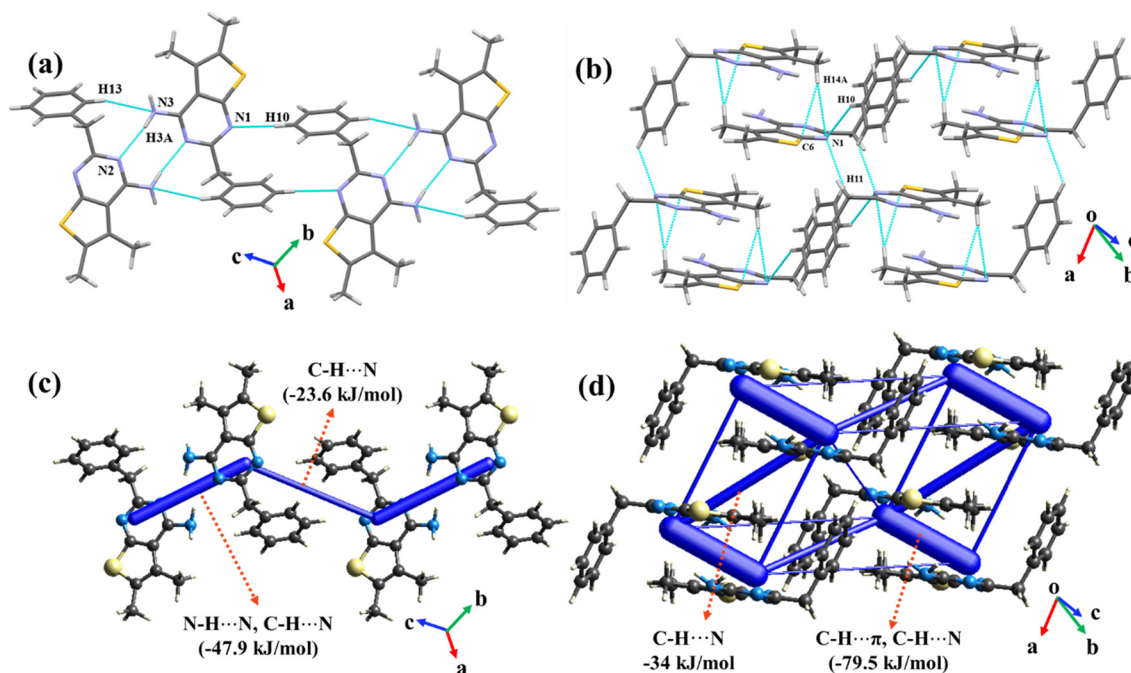
Fig. 6 (a) The packing of the molecules via N-H \cdots N and C-H \cdots N interactions (viewed down the ab -plane) in compound 6 ; (b) the herringbone structure generated through C-H \cdots N and C-H \cdots \pi interactions; (c) and (d) energy framework diagrams presenting the total interaction energy component.
