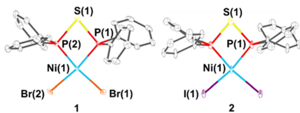
Fig. 2 Molecular structures of [\text{NiHal}_2(\text{PSP})] 1 (Hal = Br) and 2 (Hal = I). Selected bond lengths (Å) and angles ( ^\circ ) for 1 : P–S 2.1146(7)–2.1183(7) P–Ni 2.1347(6)–2.1425(6) Ni–Br 2.3271(4)–2.3370(4) P–C 1.799(2)–1.812(2) Br–Ni–Br 97.234(13) Br–Ni–P 91.613(19)–171.07(2) Ni–P–S 99.43(3)–99.80(3) P–S–P 80.81(3) P–Ni–P 79.80(2) and for 2 : P–S 2.117(3) P–Ni 2.137(3) Ni–I 2.5251(7) P–C 1.814(6)–1.816(7) I–Ni–I 100.57(8) I–Ni–P 89.93(7)–167.36(6) Ni–P–S 98.93(10) P–S–P 81.51(15) P–Ni–P 80.62(13).
