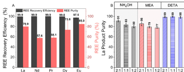
Fig. 2 (A) Recovery efficiencies and product purity for REE/Ni separation using NH 4 OH at REE:Ni of 1:2. (B) The product purity at different concentration ratios for NH 4 OH, MEA and DETA.
