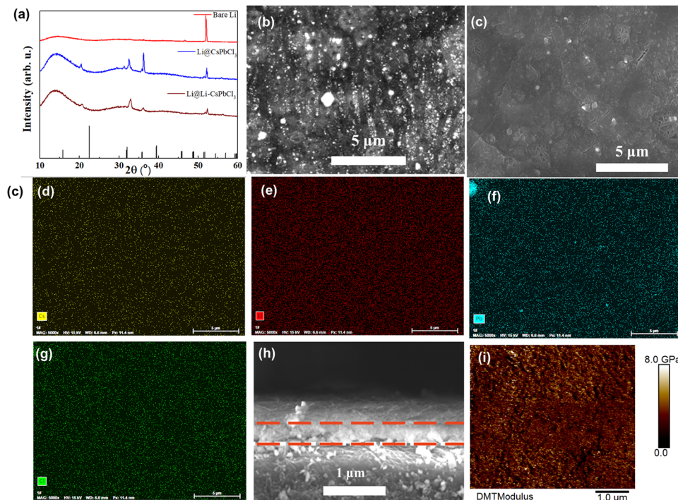
Fig. 2 (a) XRD patterns of spin-coated CsPbCl 3 and Li-CspbCl 3 on the Li foil surface. (b) and (c) SEM images of the Li-CspbCl 3 film coated on Li foil and (d)–(g) corresponding elemental mapping images of Li, Cs, Pb and Cl. (h) Cross-section SEM image of the Li-CspbCl 3 film coated on Li foil. (i) AFM Young's modulus mappings of the Li-CspbCl 3 film.
