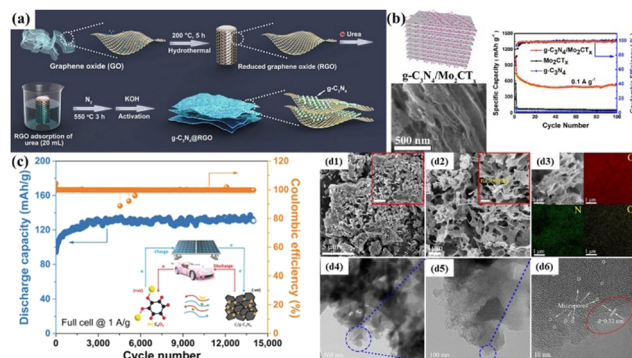
Fig. 7 (a) Procedure for the synthesis of g-C 3 N 4 @rGO. 161 Copyright 2018, the American Chemical Society. (b) Illustration and SEM images of the prepared g-C 3 N 4 /Mo 2 CT structure, together with the cycling stability of the assembled battery at a current density of 0.1 A g -1 . 166 Copyright 2021, Elsevier. (c) Configuration of a C/g-C 3 N 4 Na full cell consisting of a positive electrode of Na 2 C 6 O 6 and a negative electrode of C/g-C 3 N 4 and cycling performance of a C/g-C 3 N 4 Na full cell at 1 A g -1 . 167 Copyright 2019, Wiley-VCH. SEM images of (d1) PTI and (d2) MSGM together with high-magnification images in the inset, respectively. (d3) EDS elemental mappings and (d4)–(d6) TEM images of MSGM. 168 Copyright 2021, Elsevier.
