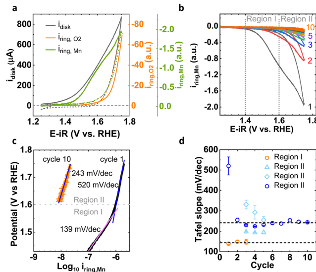
Fig. 1 (a) Cyclic voltammetry of disk current and corresponding as-measured ring current of OER and Mn dissolution for cycle 1. The anodic scan is shown as solid lines and the cathodic scan as dashed lines. (b) As-measured Mn corrosion current observed at Pt ring (potential applied at ring is 1.2 V vs. RHE) for 1st to 10th cycle and (c) Tafel slope corresponding to 1st and 10th cycle. The two distinct Mn loss processes observed before and after OER onset (above 1.6 V vs. RHE) for the 1st cycle. (d) Tafel slope as a function of number of Mn cycles.
