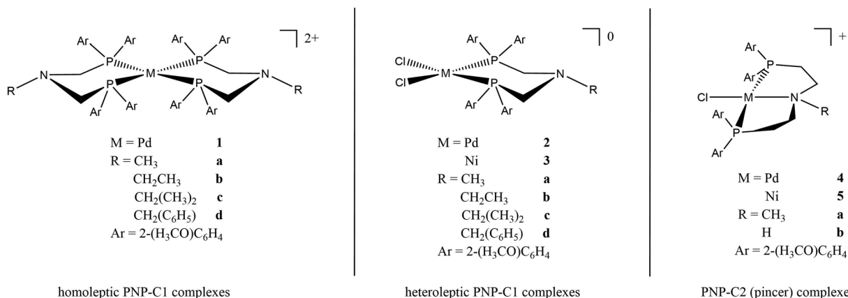
Fig. 2 Prepared complexes 1-5 with different ligands (PNP-C1-R, PNP-C2-R; R = H, Me, Et, i Pr, Bz) and metal centres (Pd, Ni). By enlarging the PNP backbone, the coordination chemistry and the mechanism of the catalytic cycle change dramatically. As is known for pincer ligands with the structure PNP-C2, a tridentate coordination is observed in contrast to the no pincer bidentate ligands of the structure PNP-C1. Thus, pincer ligands seem to stabilise complexes more, due to the five-membered ring chelate effect. In the pincer/no pincer mechanism a tridentate coordination changes to a bidentate during the catalytic cycle.
