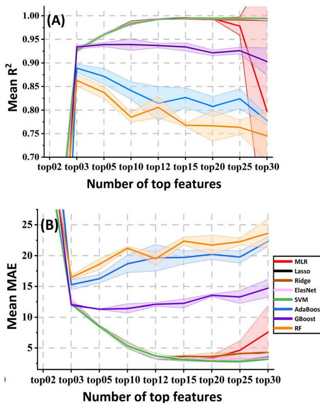
Fig. 2 The metrics changes of the pre-selected models with the different top features selected in the “Feature Importance” widget. (A) R^2 . (B) MAE. There is a large overlap between LRs and SVM.
