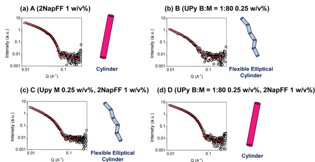
Fig. 3 Plots of SAXS data (circles) and fits (red solid lines) along with cartoon (not to scale) of structure represented by fit for (a) A (2NapFF 1 w/v%) (b) B (UPy B : M = 1 : 80, 0.25 w/v%) (c) C (UPy-M 0.25 w/v%, 2NapFF 1 w/v%) (d) D (UPy B : M = 1 : 80, 0.25 w/v%, 2NapFF 1 w/v%).
