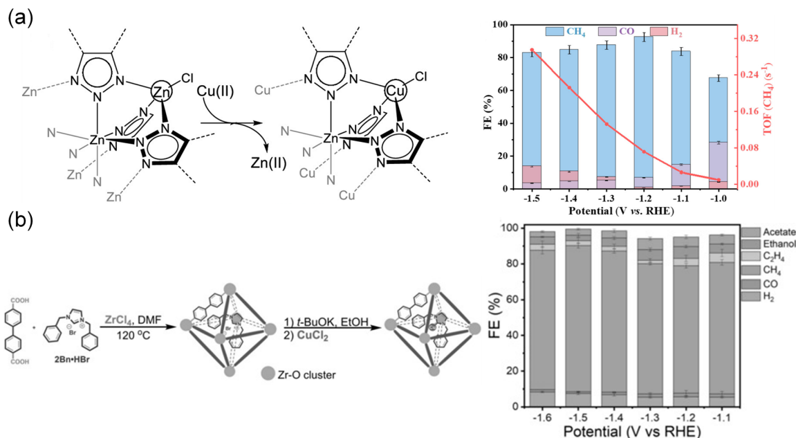
Fig. 6 (a) Schematic of the metal transformation process, and \text{FE}_{\text{CH}_4} and TOF of \text{Cu}_4\text{-MFU-4l} . 121 Copyright 2021, American Chemical Society. (b) Schematic synthesis route and FE of 2\text{Bn-Cu@UiO-67} . 120 Copyright 2021, Wiley-VCH.
