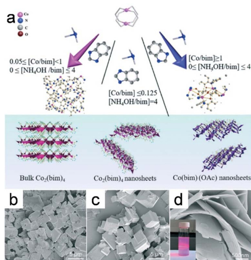
Fig. 8 (a) The diagram depicts the process for the synthesis of the Co 2 (bim) 4 , the UTCo 2 (bim) 4 , as well as the Co(bim)(OAc) prepared using varying amounts of NH 4 OH (Y value denotes the NH 4 OH/bim molar ratio): (b) Y = 0; (c) Y = 2; (d) Y = 4. (Panels a–d) Reproduced with permission. 19 Copyright 2019, Royal Society of Chemistry.
