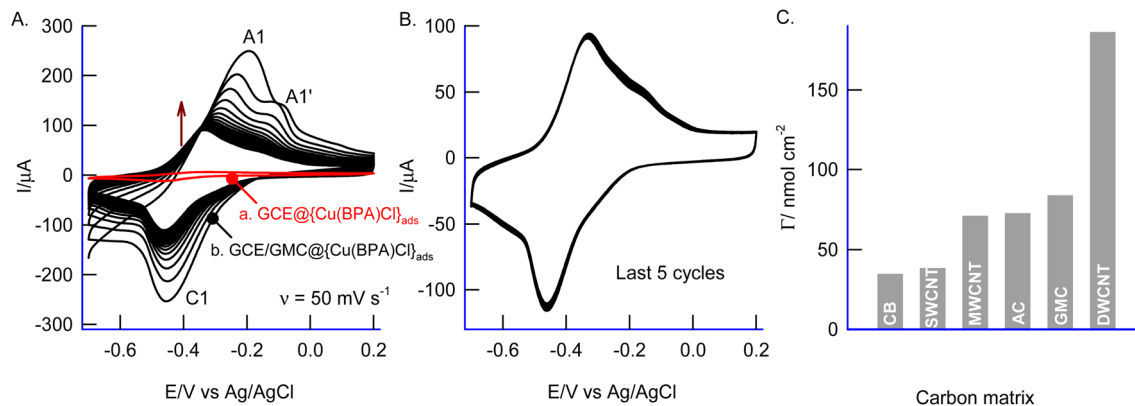
Fig. 1 (A) Cyclic voltammograms of (a) GCE@{Cu(BPA)Cl} ads ; (b) GCE/GMC@{Cu(BPA)Cl} ads in nitrogen purged 0.1 M PBS, pH 7, at scan rate ( \nu ) = 50 mV s -1 ( n = 20 cycles) and (B) last five CVs; (C) comparative plots of surface excess values of different carbon nanomaterials used.
