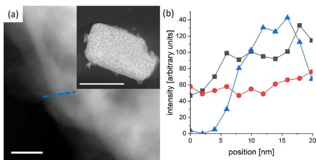
Fig. 5 LaTiO 2 N particle scratched from a PEC electrode after 21 h operation. (a) High angle annular dark field scanning TEM image of the edge (scale bar 20 nm) of a particle (see inset scale bar 1 \mu m) (b) combined scanning TEM EDX/EELS profile along the blue line indicated in (a) triangles in blue denote N K-edge (EELS), black squares and red dots the La L \alpha and Ti K-edge respectively (EDX). The N content is reduced close to the particle edge with respect to the bulk.
