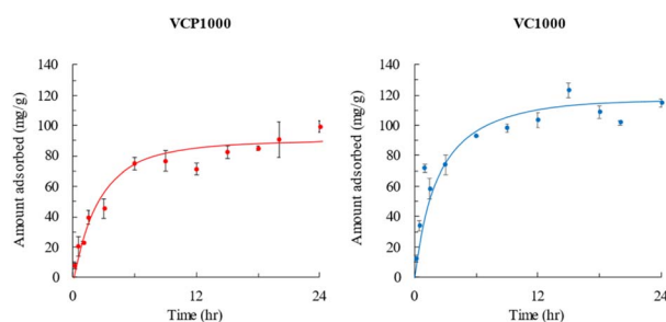
Fig. 5 The effect of contact time on the adsorption of CV onto VCP1000 or VC1000. Initial concentration, 100 mg L -1 ; sample volume, 50 mL; adsorbent, 0.02 g; temperature, 25 °C; contact time, 10 and 30 min and 1, 1.5, 3, 6, 9, 12, 15, 18, 20, and 24 h, 100 rpm.
