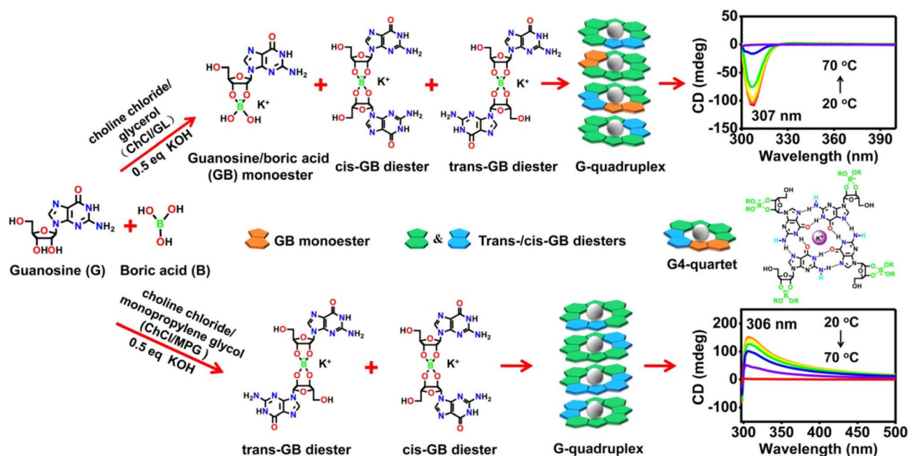
Fig. 14 The reaction of guanosine with H_3BO_3 and KOH in different DESs produced different species distribution and drove the chiral self assembly of the G-quadruplex with opposite chiroptical features. Reprinted with permission from C. Gu, Y. Peng, J. Li, H. Wang, X. Q. Xie, X. Cao and C. Sen Liu, Supramolecular G4 Eutectogels of Guanosine with Solvent-Induced Chiral Inversion and Excellent Electrochromic Activity, Angew. Chem., Int. Ed. , 2020, 59, 18768–18773. Copyright 2020 Wiley-VCH GmbH.
