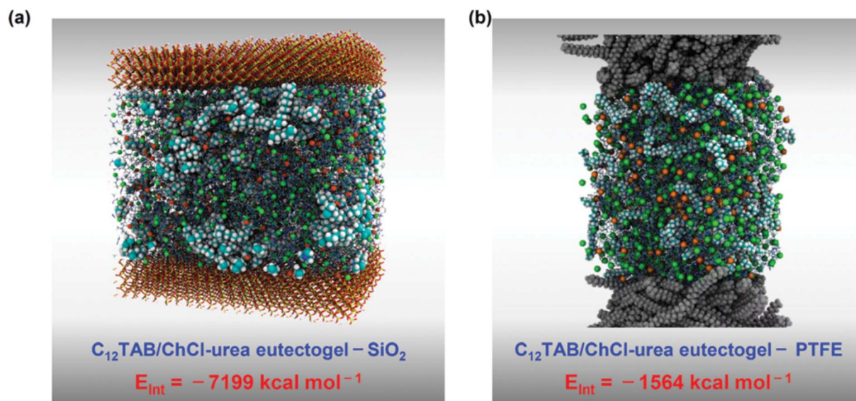
Fig. 24 Left: minimized structure of C 12 TAB/ChCl–U confined between two layers of glass (a) and PTFE (b). The interaction energy E_{\text{int}} clearly shows stronger adhesion on glass than PTFE, due to the larger coulombic contribution in the former compared to the latter. Reproduced from Y. Liang, K. Wang, J. Li, Y. Zhang, J. Liu, K. Zhang, Y. Cui, M. Wang and C. Sen Liu, Low-molecular-weight supramolecular adhesives based on non-covalent self-assembly of a small molecular gelator, Mater. Horiz. , 2022, 9, 1700–1707 with permission from the Royal Society of Chemistry.
