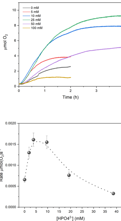
Fig. 4 (Top panel) O 2 evolution kinetics (see Table 2 for conditions). (Bottom panel) Plot of \text{Rate}(\text{O}_2)_{\text{MAX}} vs. the concentration of \text{HPO}_4^{2-} buffer base. Error bars result from repetitive runs.
