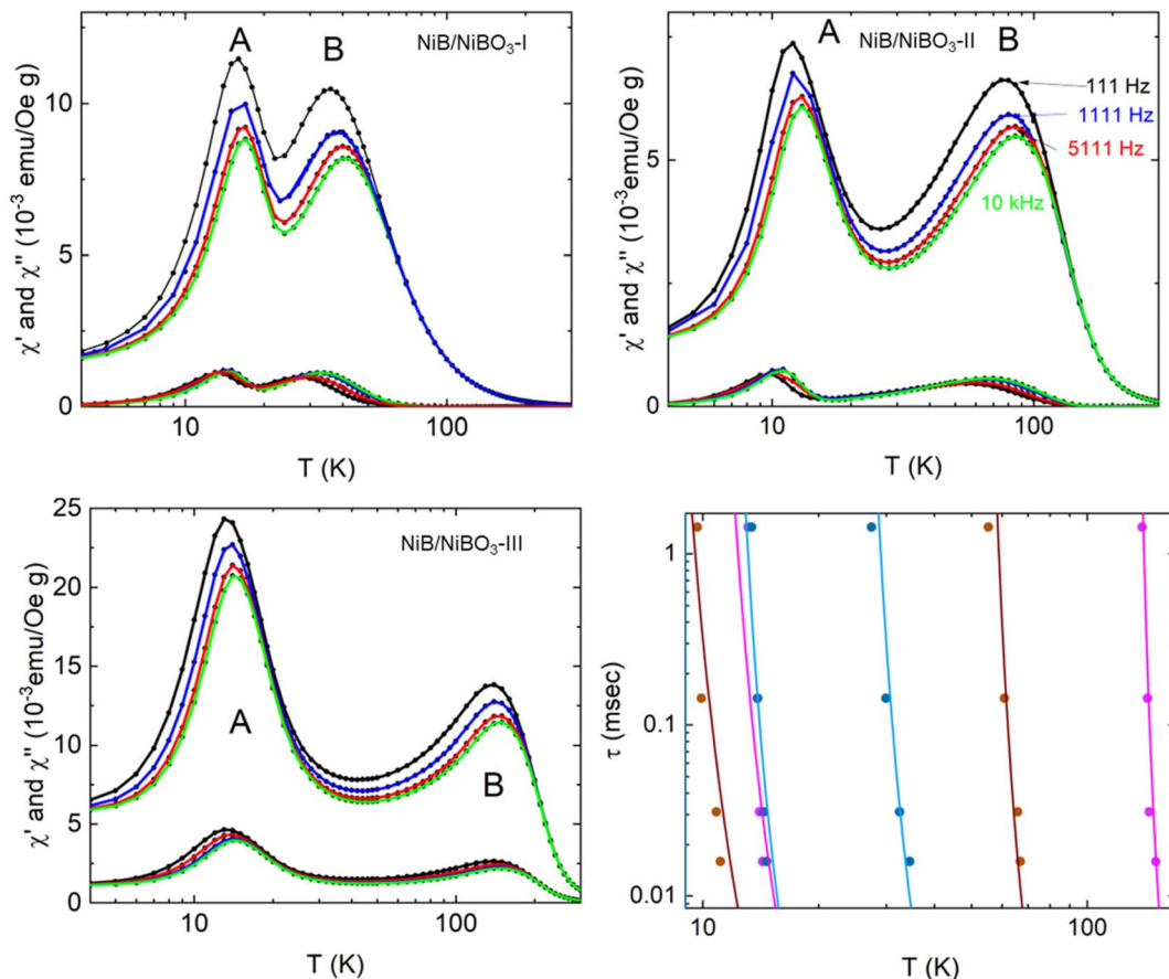
Fig. 6 Temperature variation of the real and imaginary fundamental magnetic ac-susceptibility for NiB/NiBO 3 -I, NiB/NiBO 3 -II, and NiB/NiBO 3 -III samples. The data are collected with an amplitude of the ac-magnetic field 5 Oe and frequencies f = 111 Hz, 1111 Hz, 5111 Hz, and 10 kHz. Temperature variation of the relaxation times for the two peaks observed in the three samples. The Vogel-Fulcher empirical equation reproduces the solid lines using the parameters listed in Table 4.
