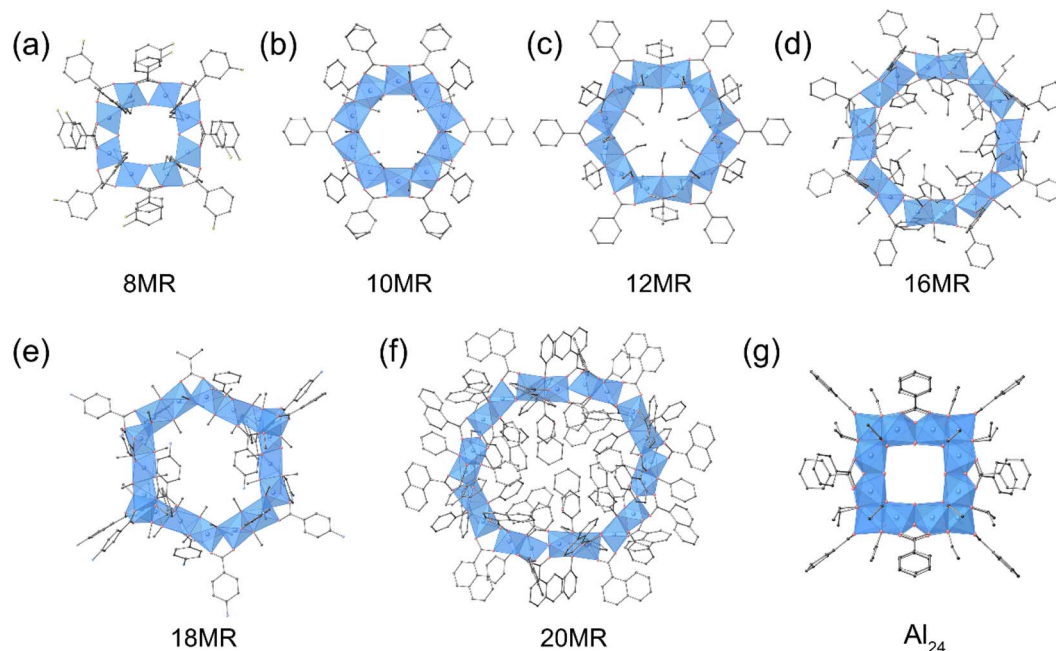
Fig. 2 Molecular structure of (a) [\text{Al}_8(\text{OH})_4(3\text{-fluorobenzoate})_{12}(\text{O}i\text{Bu})_8] (8MR), (b) [\text{Al}_{10}(\text{benzoate})_{10}(\text{OMe})_{20}] (10MR), (c) [\text{Al}_{12}(\text{benzoate})_{12}(\text{O}i\text{Pr})_{24}] (12MR), (d) [\text{Al}_{16}(\text{OH})_8(\text{benzoate})_{24}(\text{OPr}^n)_{16}] (16MR), (e) [\text{Al}_{18}(4\text{-aminobenzoate})_{18}(\text{OMe})_{36}] (18MR), (f) [\text{Al}_{20}(\text{phenol})_{20}(\text{OH})_{10}(1\text{-naphthalenecarboxylate})_{30}] (20MR), and (g) [\text{Al}_{24}(\text{BA})_{12}(\text{EtO})_{24}(\text{OH})_{32}]^{4+} ( \text{Al}_{24} ).
