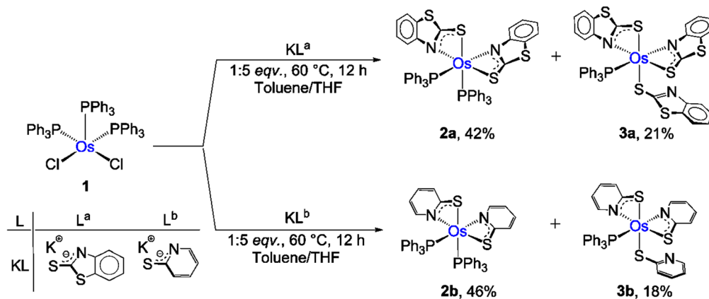
Scheme 1 Syntheses of Os(II) and Os(III)- N,S -chelated complexes.
