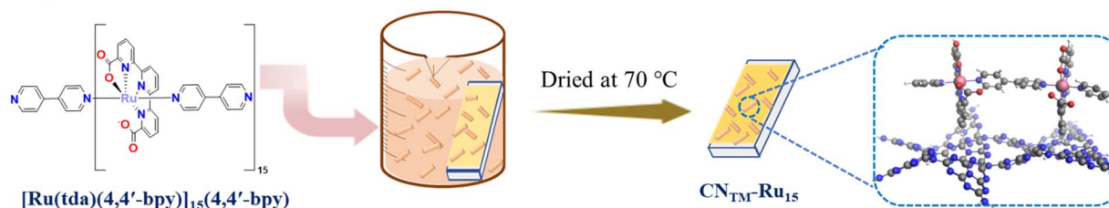
Scheme 1 Procedure for the preparation of a CN TM film and the anchoring of the Ru 15 oligomer to generate the hybrid material CN TM -Ru 15 .
