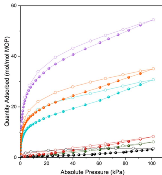
Fig. 4 Isotherms of CO_2 -adsorption at 195 K for the deprotected (N_3)_1 -RhMOP (green), the deprotected (alkyne) 1 -RhMOP (red), the (alkyne) 24 -RhMOP (black), the MOP-dimer (purple), the MOP-tetramer (blue), and the MOP-satellite (orange).
