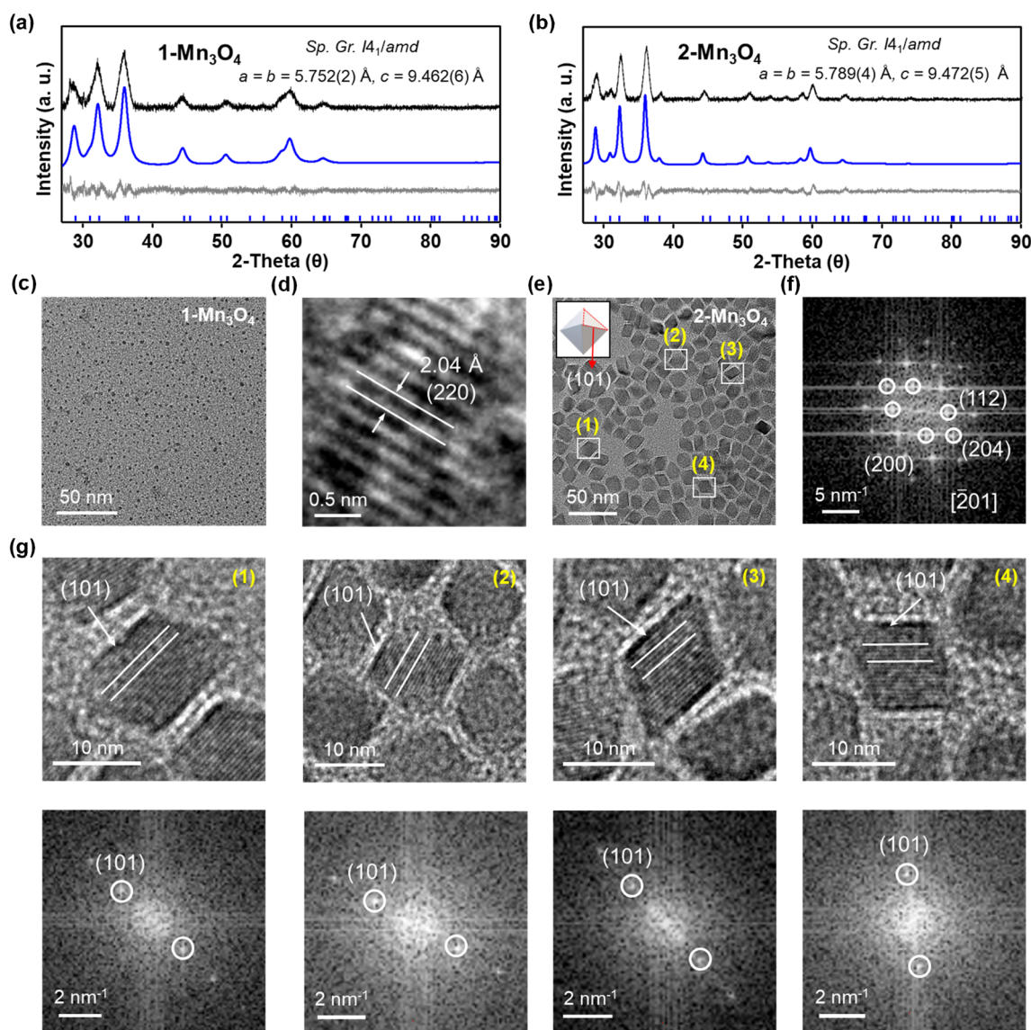
Fig. 7 (a) and (b) X-ray powder diffraction patterns and Le Bail fit for Mn 3 O 4 nanocrystals obtained from [Mn 18 -Ac] and [Mn 18 -Piv]. Black and blue curves are experimental and simulated patterns with theoretical positions shown at the bottom as blue bars. The grey is the difference curve. (c) and (d) TEM micrographs of 1-Mn 3 O 4 nanocrystals obtained from [Mn 18 -Ac]. (e) TEM micrographs of the Mn 3 O 4 nanocrystals obtained from [Mn 18 -Piv]. Inset graph is the schematic representation of the octahedron geometry for 2-Mn 3 O 4 nanocrystals. (f) Fast Fourier transform (FFT) pattern for the TEM micrograph of the 2-Mn 3 O 4 nanocrystals from the view of [201] orientation. (g) High-resolution TEM micrographs (top) of selected nanocrystals in (e) and the corresponding fast Fourier transform (FFT) patterns (bottom).
