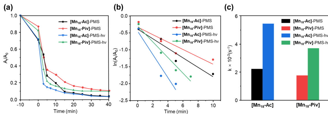
Fig. 6 TC degradation rates over reaction time (a) and the pseudo-first-order kinetic modeling (b) for the catalytic behavior of [Mn_{18}\text{-Ac}] and [Mn_{18}\text{-Piv}] clusters under dark condition and light irradiation; (c) histogram of the degradation rate constant for [Mn_{18}\text{-Ac}] and [Mn_{18}\text{-Piv}] under dark environment and light irradiation.
