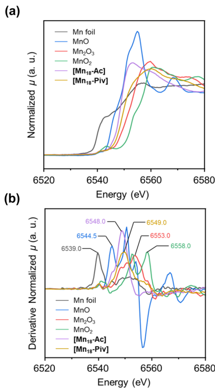
Fig. 5 Normalized XANES spectra (a) and the first-derivative normalized XANES spectra (b) for Mn^0 foil, Mn^{II}O , Mn^{III}_2O_3 , Mn^{IV}O_2 , [Mn_{18}\text{-Ac}] , and [Mn_{18}\text{-Piv}] .
