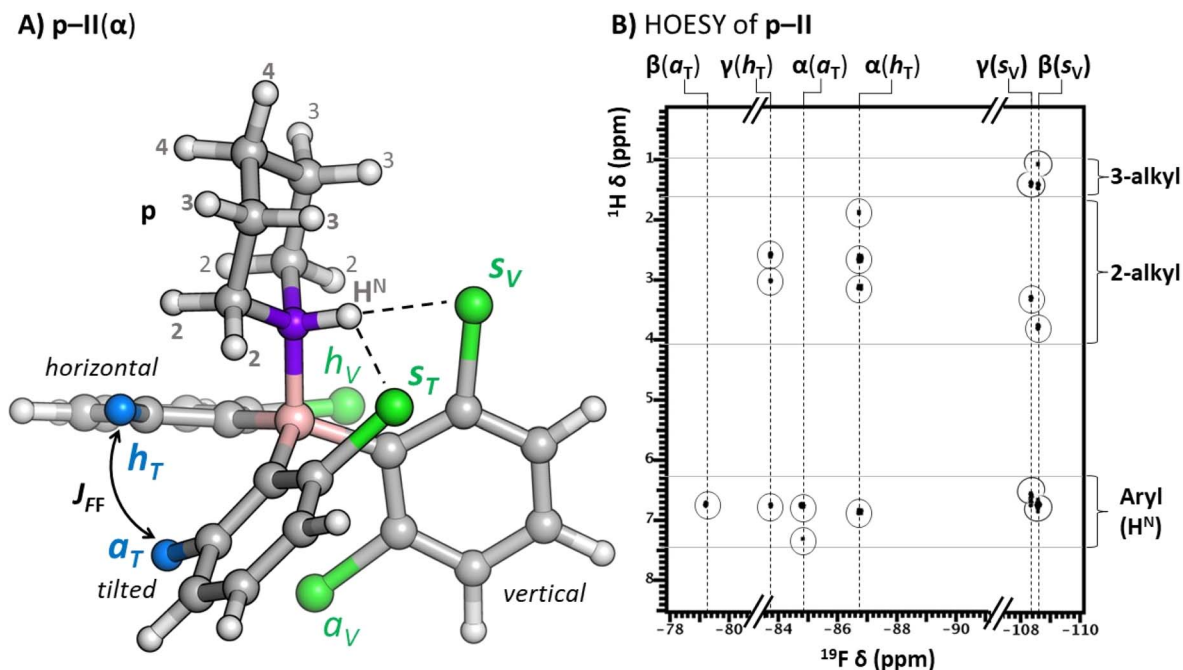
Fig. 6 (A) The common ring topology of the computed p -adduct structures illustrated with the lowest lying (α) conformation of p -II. The emerging halogen atom positions are denoted as horizontal ( h ), syn ( s ) or anti ( a ) whereas the subscripts specify whether the halogen atom is located on ( s , a ) or points towards ( h ) the tilted (T) or vertical (V) ring. The hydrogen bonding interaction between the H N and the syn-positioned ligands is indicated with black dashed lines. The p -II(α) features the two F atoms (blue) in the a T and h T positions through which a through-space J FF coupling of 39.5 Hz emerges (see α( a T ) and α( h T ) signals in Fig. 5). (B) The 19 F- 1 H HOESY correlations of the p -II atropisomers (α, β and γ) are highlighted with circles. The s -fluorines (of the β and γ atropisomers) are found sufficiently close in space to most of the p ring to be correlated with the H N and most of the alkyl p hydrogens; the h -fluorines (α, γ) are correlated with a limited number of alkyl p hydrogens; in contrast, the a -fluorines (α and β) do not display HOESY contacts with p .
