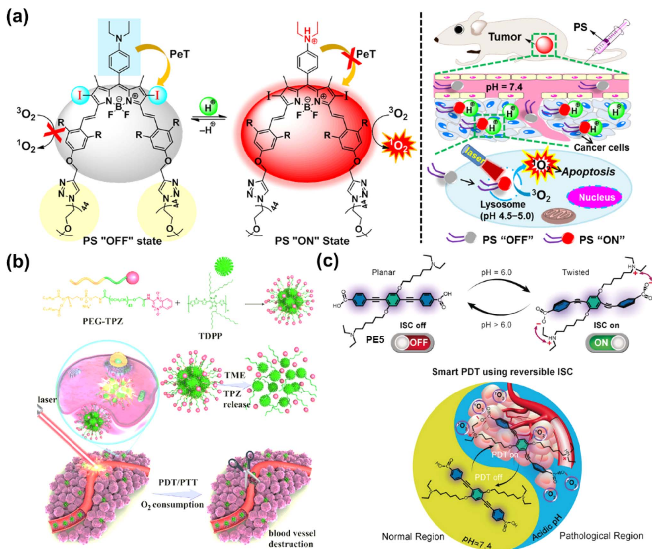
Fig. 8 (a) The pH-activatable BODIPY derivative for 1 O 2 generation and PDT. Reproduced with permission from ref. 82. Copyright 2018 American Chemical Society. (b) Illustration of the TDPP@PEG-TPZ nanoformulation for phototherapy-enhanced chemotherapy. Reproduced with permission from ref. 83. Copyright 2023 The Royal Society of Chemistry. (c) Reversible switching of ISC and potential application in PDT. Reproduced with permission from ref. 84. Copyright 2019 Wiley-VCH.
