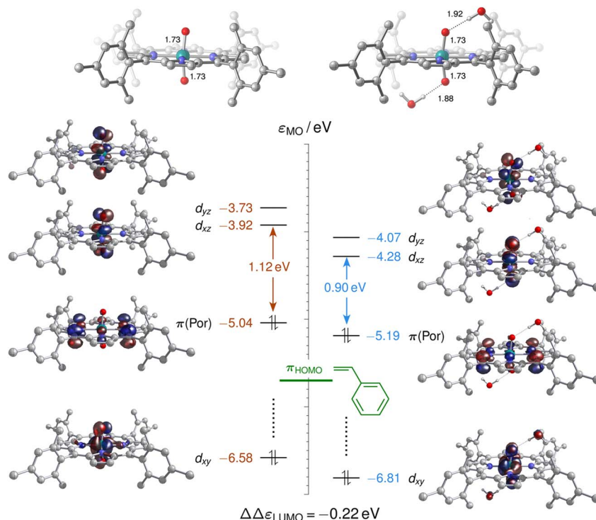
Fig. 11 Molecular orbital energy diagram (eV) for [(\text{L1})\text{Ru}^{\text{VI}}(\text{O})_2]_2 , ^1\text{A} (left), and [(\text{L1})\text{Ru}^{\text{VI}}(\text{O})_2]_2 \cdot (\text{H}_2\text{O})_2 , ^1\text{A}_{\text{w2}} (right), showing selected frontier orbitals computed at the M06L-D3(SMD)/def2TZVP level. The relative stabilisation \Delta\epsilon_{\text{LUMO}} of the lowest unoccupied molecular orbital (LUMO) is computed with reference to the corresponding highest occupied molecular orbital (HOMO), which is orthogonal to the \text{O}=\text{Ru}=\text{O} axis. \Delta\epsilon_{\text{LUMO}} is equivalent to the difference of the HOMO/LUMO gaps, and the horizontal green bar at -5.7 eV indicates the HOMO energy level of styrene.
