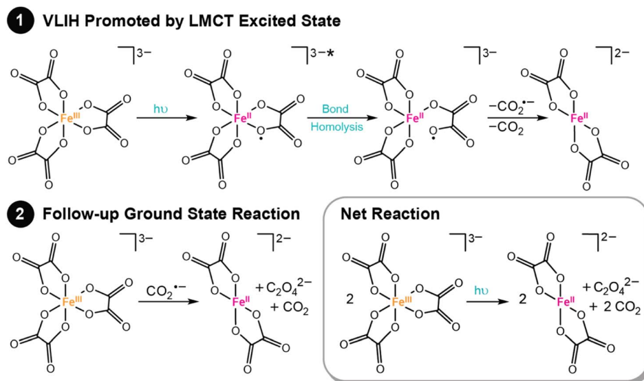
Fig. 3 VLIH mechanism of ferrioxalate to form ferrous oxalate. Further decomposition of the C_2O_4^{\bullet -} with a second equivalence of ferric oxalate yields an additional equivalence of ferrous oxalate and two equivalents of CO_2 .
