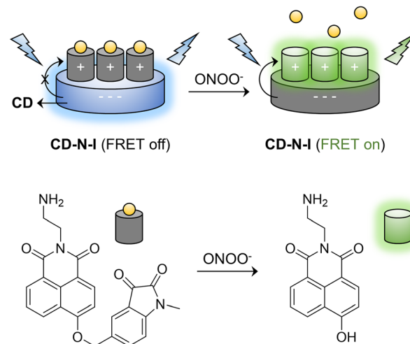
Scheme 1 Schematic diagram of the mechanism of peroxynitrite detection using CD-N-I.
