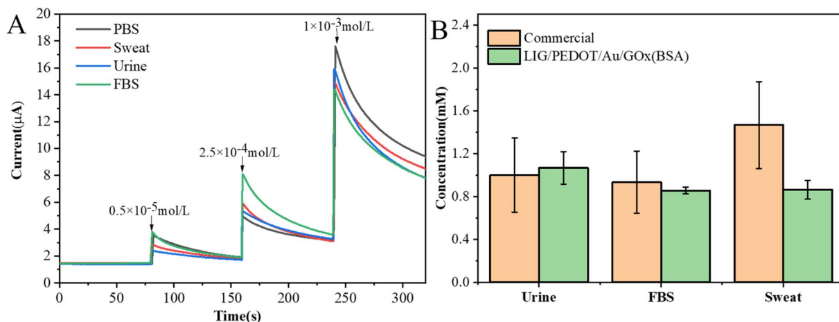
Fig. 10 (A) i - t curves of actual samples with different concentrations of glucose; (B) comparison of the measured glucose in actual samples between the commercial and our LIG-based flexible glucose sensors.
