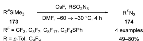
Scheme 52 Synthesis of azidoperfluoroalkanes 174 through nucleophilic fluoroalkylation of sulfonyl azides.
