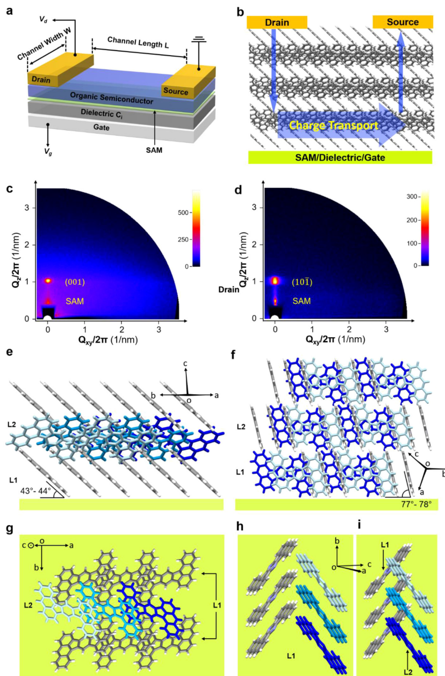
Fig. 7 Molecular orientation of DBAF and DBAF- N_2 at the organic/SAM/inorganic interface of the OTFT devices. (a) The OTFT device used in this work has a bottom-gate-top-contact structure. (b) Illustration of charge transport taking place in a working device of DBAF. (c) and (d) are typical GIWAXS data for the DBAF- and DBAF- N_2 -based devices, respectively. (e) Side view and (g) top view of the orientation of DBAF molecules. (f) Side view and (h and i) top views of the orientation of DBAF- N_2 molecules. (h) shows the first layer (L1) at the SAM/inorganic substrate (bright green). (g) and (i) show the first two layers, in which molecules colored in grey come from the first layer (L1) and molecules in various blue colors are from the second layer (L2).
