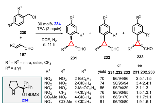
Scheme 52 MIRC cyclopropanation of benzyl chlorides and \alpha,\beta -unsaturated aldehydes using catalyst 234 .
