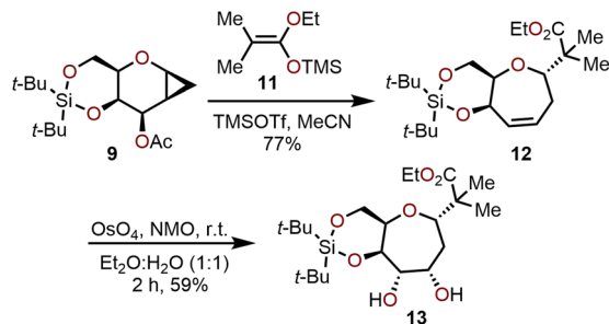
Scheme 3 Advancement of cyclopropanated sugar 9 toward polyoxy-generated oxepanes through Hoberg's ring-expansion protocol and dihydroxylation. 10
