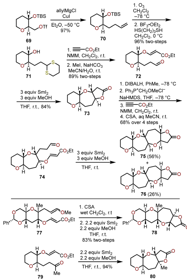
Scheme 14 \text{SmI}_2 mediated radical cyclization strategy toward fused polyoxygenated oxepanes. 32,34
