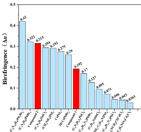
Fig. 4 Comparison of the birefringence of the hybrid metal halide perovskites.
