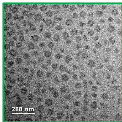
Fig. 10 SAXS (at C = 50 \text{ g L}^{-1} ) and cryo-TEM (at C = 30 \text{ g L}^{-1} ) monitoring the progressive protonation of the AA units in the B block of sample A-1 (spheres, F_{AA} = 0.02 , gradient). The black dotted lines are models fitting the data (see Table S7†).
