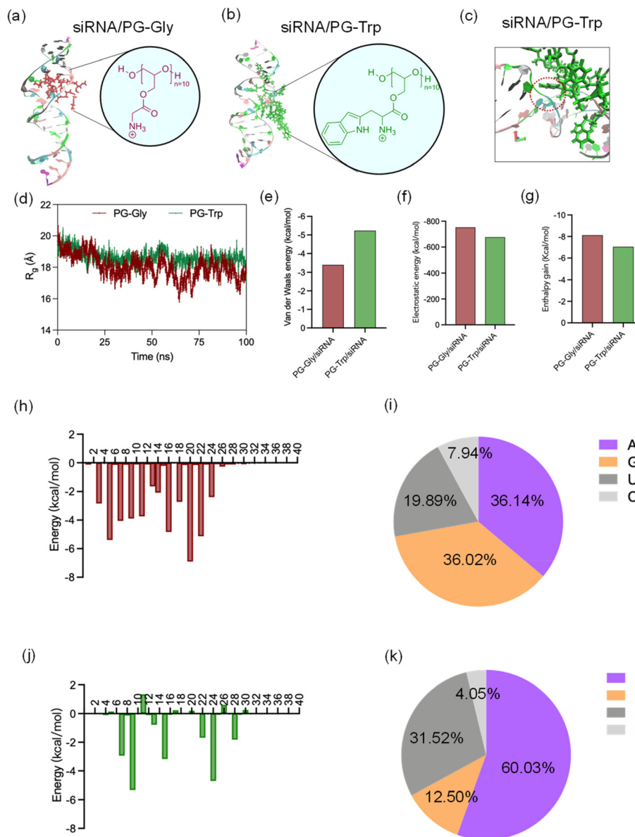
Fig. 4 Molecular dynamics (MD) simulation of siRNA binding with polycations. Front view snapshots taken from the dynamic simulation of PGGly/siRNA (a) and PGTrp/siRNA (b). Zoomed front view snapshots taken from the dynamic simulation of PGTrp/siRNA (c). Time evolution of Radius of gyration ( R_g ) of PGGly/siRNA and PGTrp/siRNA systems (d). van der Waals energy (e), electrostatic energy (f) and enthalpy gain (g) during polymers/siRNA interaction (normalized per charged amine, expressed in kcal mol -1 ). Molecular Mechanics/Poisson-Boltzmann Surface Area (MM/PBSA) per-residue energy decomposition analysis of siRNA-polymer complex ((h)–(k)). Nucleotide energy contribution spectrum in PGGly/siRNA interaction (h) and percentages of four bases contribution (i). Nucleotide energy contribution spectrum in PGTrp/siRNA interaction (j) and percentages of four bases contribution (k).
