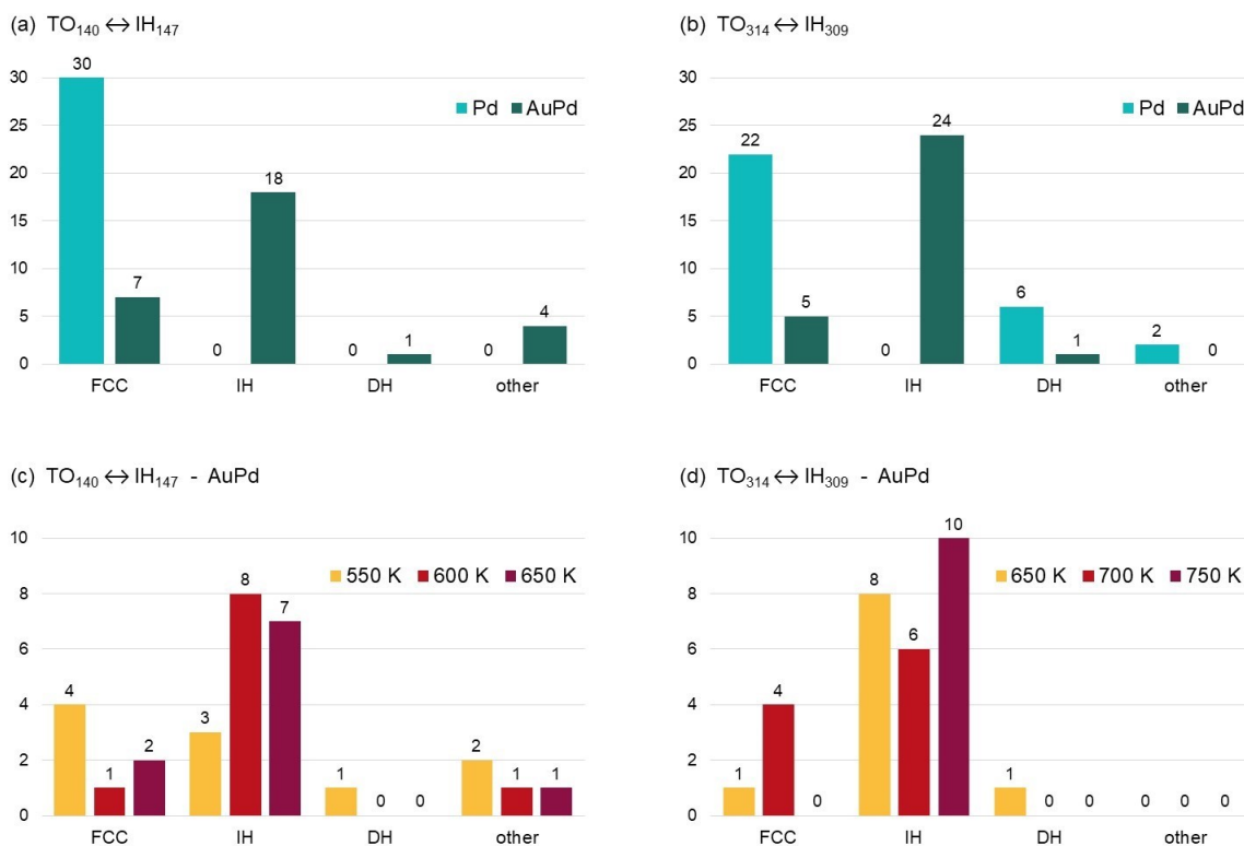
Fig. 2 Frequency of the different structural motifs, namely crystalline (FCC), noncrystalline icosahedral (IH) and decahedral (DH) motifs, at the end of the (a) TO_{140} \leftrightarrow IH_{147} and (b) TO_{314} \leftrightarrow IH_{309} coalescence simulations, for both pure Pd and \sim 20\% Au compositions. "Other" structures include bi- and tri-decahedra, i.e. with 2 or 3 converging five-fold symmetry axes, 10,31 and kinetically-trapped configurations in which the initial subunits are still well-distinguishable. (c,d) Frequency of the different structural motifs in the AuPd cases, for the three simulation temperatures.
