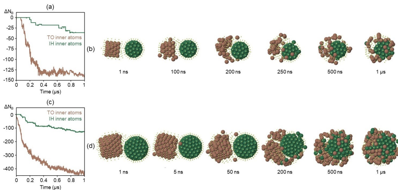
Fig. 9 Mobility of TO and IH inner atoms in two representative simulations ending up with the IH structural motif. (a-b) \text{TO}_{140} \leftrightarrow \text{IH}_{147} , AuPd composition, 650 K. (c-d) \text{TO}_{314} \leftrightarrow \text{IH}_{309} , AuPd composition, 750 K. Simulations are the same as in Figure 4. (a,c) Evolution of \Delta N_B during the whole simulation. (b,d) Snapshots of the simulations, in which atoms are coloured according to their position before the collision: brown - atoms initially belonging to the inner part of the TO; green - atoms initially belonging to the inner part of the IH. All other atoms are displayed as small spheres.
