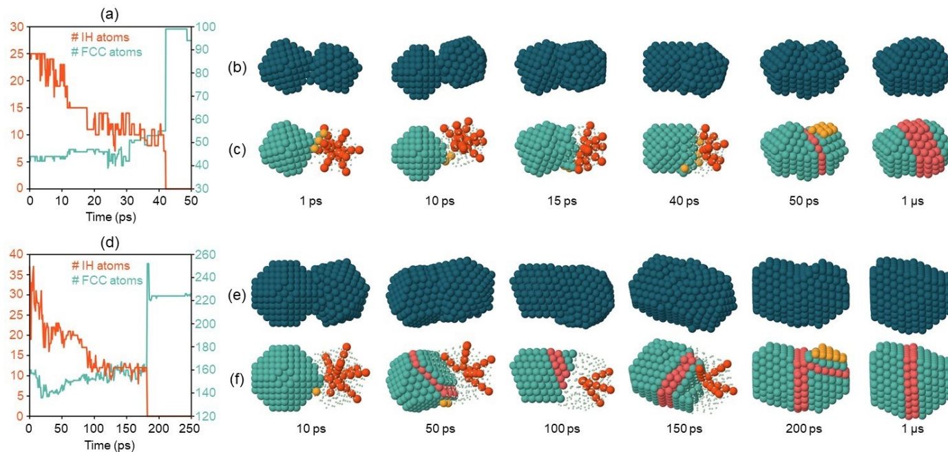
Fig. 4 Representative simulations ending up with the FCC structural motif. (a-c) TO_{140} \leftrightarrow IH_{147} , pure Pd composition, 600 K. (d-f) TO_{314} \leftrightarrow IH_{309} , pure Pd composition, 700 K. (a,d) Evolution of the number of atoms with IH and FCC local environment, in the first part of the simulation. (b,e) Snapshots of the simulations in the same time range, and at the end of the simulations. (c,d) Same snapshots as in (b,e), but atoms are coloured according to their local environment: light blue - closed-packed planes in fcc stacking; orange - five-fold symmetry axes; pink - closed-packed planes in hcp stacking; yellow - surface planes in stacking fault. All other atoms are displayed as small spheres.
