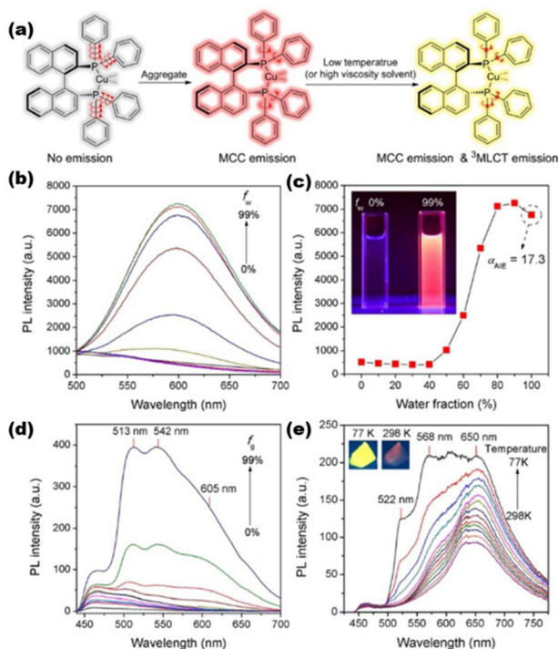
Fig. 3 (a) RIM mechanism of the \text{R/S-Cu}_3 nanocluster; (b) emission spectra of \text{R/S-Cu}_3 in \text{DMSO-H}_2\text{O} mixtures with different ratios; (c) emission intensity of \text{R/S-Cu}_3 at 605 nm as a function of the volume fraction of water ( f_w ); (d) emission spectra of \text{R/S-Cu}_3 in \text{EtOH-glycerol} mixtures with different f_g values; and (e) temperature-dependent emission spectra of \text{R/S-Cu}_3 in the solid state. Reproduced from ref. 99 with permission from Wiley, copyright (2020).
