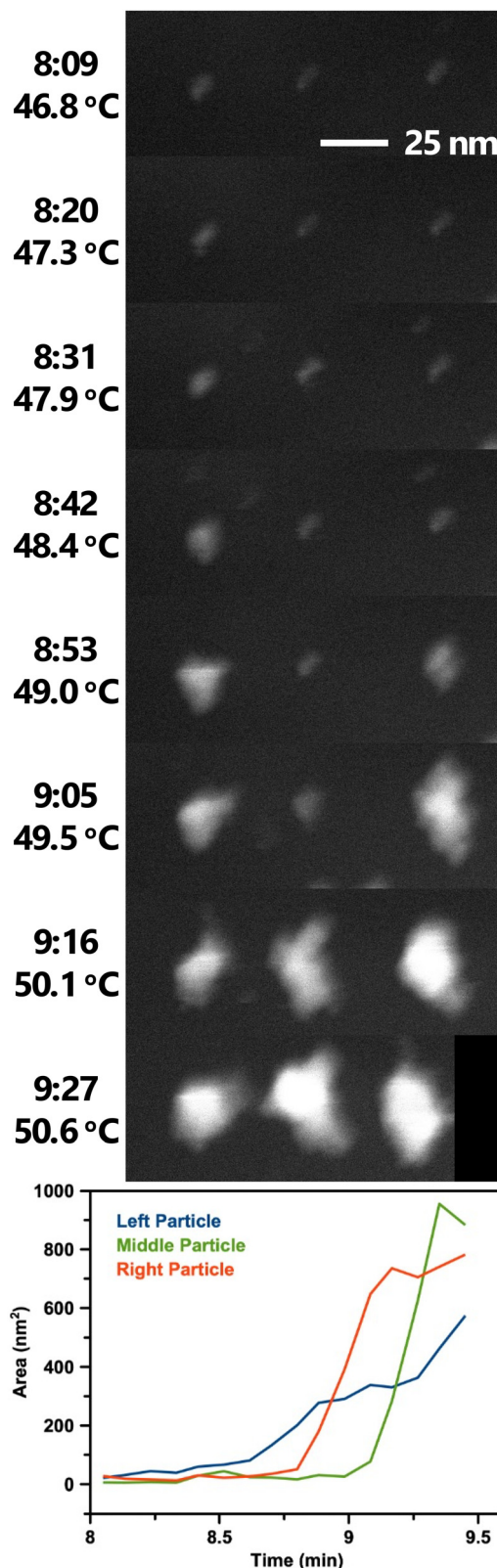
Fig. 7 Selected STEM images from Movie 2† showing BiOCl formation and growth from BiCl 3 Lac. Images are spaced ca. 11 s apart with times and temperatures indicated. The black area in the last frame is where the particle clusters drifted near the edge of the field of view and was applied during drift correction. Scale bar applies to all images. Below the images is a plot of the clusters' 2D area over time. Image processing steps for Movie 2 are shown in Movie S1†
