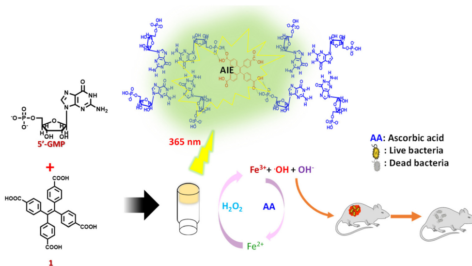
Scheme 1 Supramolecular hydrogels mediated by the crosslinking of GMP with 1 and divalent metal ions (M) as in M- 1_{\text{GMP}} to exhibit aggregation-induced emission. The \text{Fe}-1_{\text{GMP}} hydrogel exhibits upregulation of the Fenton reaction in the presence of ascorbic acid to generate ROS for eventual application in controlling bacterial growth in topical wounds.
