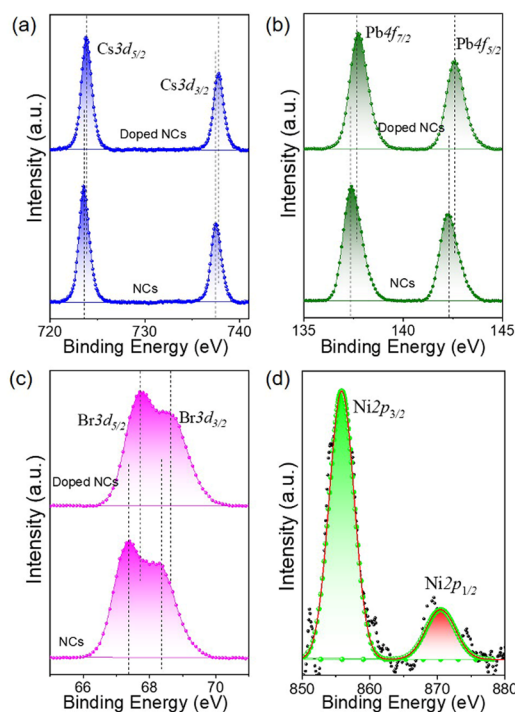
Fig. 2 Survey scans of the oxidation states of elements in the XPS spectra of both pristine and doped \text{CsPbBr}_3 NCs, which show (a) Cs-3d, (b) Pb-4f, and (c) Br-3d orbitals. The upper and lower panels show the XPS spectra of \text{Ni}^{2+} -doped \text{CsPbBr}_3 and \text{CsPbBr}_3 NCs, respectively. (d) XPS spectrum of Ni-2p orbitals.
