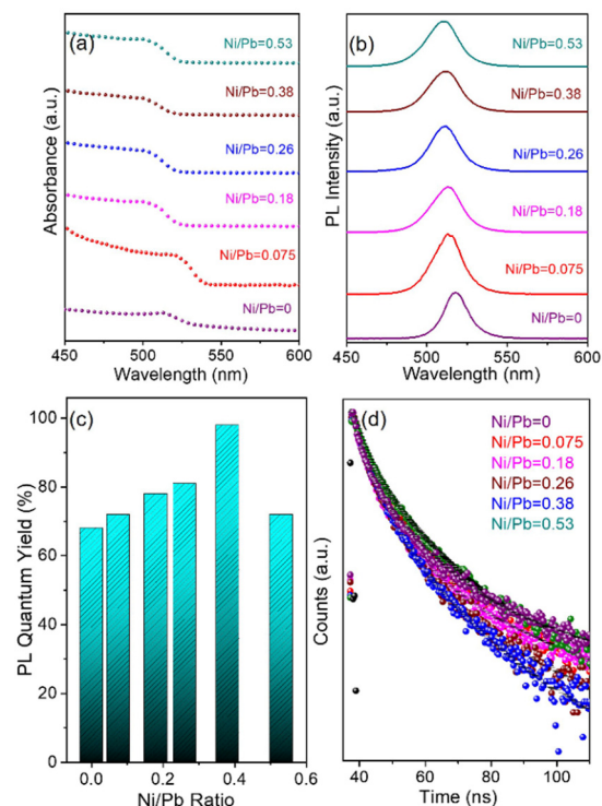
Fig. 4 (a) UV-vis absorption spectra and (b) variation in the PL spectra upon changing the doping concentration of \text{Ni}^{2+} ions. (c) PLQYs with increasing dopant concentration. (d) Time decay curves with doping concentration variation. The legends used in the figure represent the elemental ratio of Ni/Pb obtained from ICP-AES.
