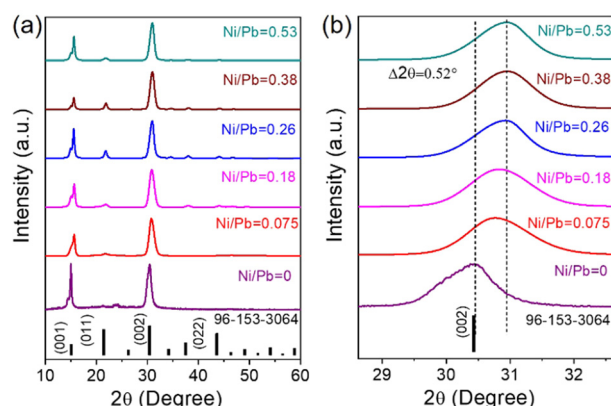
Fig. 3 (a) XRD patterns with changing \text{Ni}^{2+} concentration showing the cubic perovskite phase (COD file: 96-153-3064). (b) Enlarged XRD patterns showing a red shift of diffracting peaks with increasing \text{Ni}^{2+} concentration. The legends used in the figure represent the elemental ratio of Ni/Pb obtained from ICP-AES.
