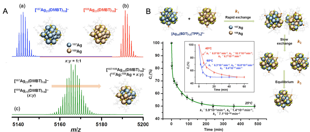
Fig. 12 (A) ESI MS of (a) [^{107}\text{Ag}_{25}(\text{DMBT})_{18}]^- , (b) [^{109}\text{Ag}_{25}(\text{DMBT})_{18}]^- , and (c) isotopically mixed [\text{Ag}_{25}(\text{DMBT})_{18}]^- nanocluster with ^{107}\text{Ag} : ^{109}\text{Ag} ratio of 1 : 1. (B) Kinetics of isotopic Ag atom exchange in [\text{Ag}_{25}(\text{BDT})_{12}(\text{TPP})_4]^{3-} nanocluster. Adapted from ref. 272. Copyright 2019 American Association for the Advancement of Science.
