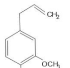
Eugenol
