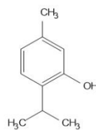
Thymol
