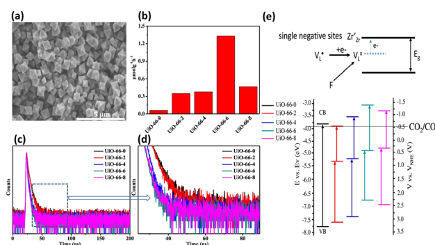
Fig. 6 (a) SEM images of UiO-66-6 and UiO-66-0 (inset). (b) Results of CO 2 production from photocatalytic CO 2 production under visible light illumination over various UiO-66- X . (c and d) Time-resolved PL spectra of various UiO-66- X . (e) Proposed mechanism of the energetic state of missing ligands and derived band structure for various UiO-66- X ( X = 0, 2, 4, 6, 8). Reproduced with permission from ref. 43. Copyright 2022, American Chemical Society.
