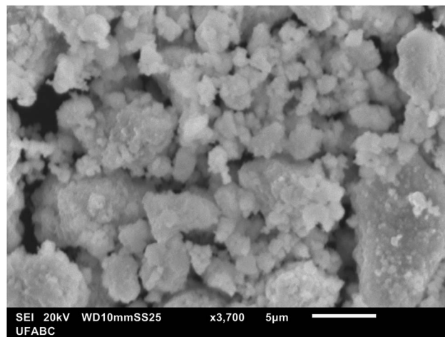
Fig. 5 SEM image of the \text{Cs}_2\text{SbAgCl}_6 polycrystalline material. The scale bar at the lower right of the SEM image is between 5 \mu\text{m} on a 3.700 \times magnification scale.
